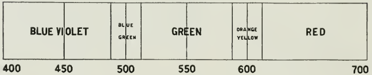
Fig. 102. Divisions of Spectrum.
